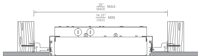
Trim or Trimless (mud-in) Flange Kit
